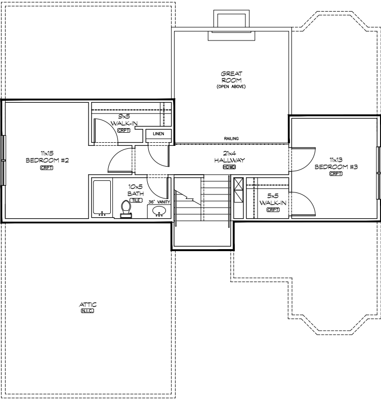
2nd Floor 595 sq. ft.
